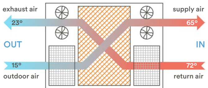
Fig 1. During winter, heat from the return air is transferred to the supply air in the heat recovery core (orange hatch) of an ERV. The flow of heat reverses in summer, where heat from the outdoor air is transferred to the exhaust air, helping to cool the supply air.
