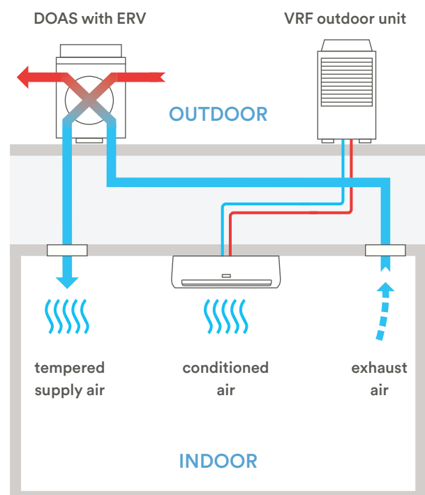
Fig 2. When paired with a VRF heating and cooling system, a DOAS with ERV creates a complete HVAC solution. In cooling mode, for instance, the ERV uses the exhaust air to transfer heat from the outdoor air, tempering the supply air to the building. The VRF does less work because the supply air temperature from the DOAS is closer to the desired indoor temperature.
